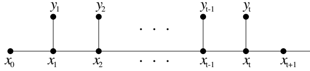
FIGURE 3.4. A graphical representation of the state-space model, also called the hidden Markov model (HMM).
