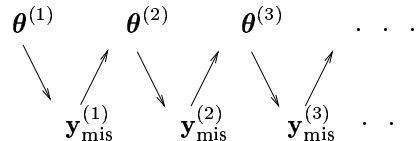
FIGURE 6.2. A graphical illustration of the data augmentation scheme.
