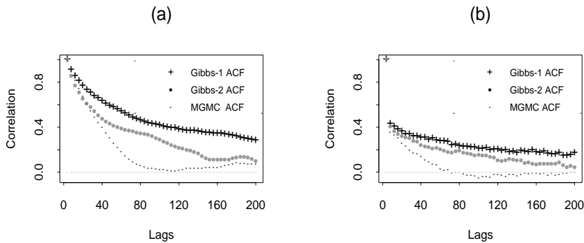
FIGURE 8.9. The Gibbs sampler's lag-1 and lag-2 versus multigrid Monte Carlo's lag-1 autocorrelation functions (a) for \sigma and (b) for \beta .
