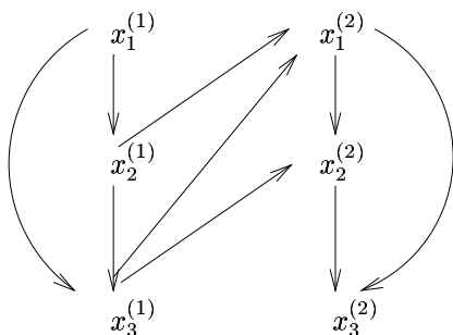
FIGURE 6.4. A graphical illustration of the standard Gibbs sampler with three components. The arrows represent the “causal relationships” in Gibbs sampling: x_1^{(2)} is drawn conditional on (x_2^{(1)}, x_3^{(1)}) ; x_2^{(2)} is drawn conditional on (x_3^{(1)}, x_1^{(2)}) ; and x_3^{(2)} is drawn conditional on (x_1^{(2)}, x_2^{(2)}) .
