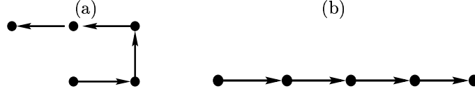
FIGURE 3.3. Two different configurations for SAW with N = 5 nodes. (a) and (b) have different sampling probabilities according to the Rosenbluth method.
