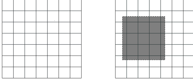
FIGURE 8.1. Left: an 8 \times 8 lattice \Lambda ; Right: a 4 \times 4 sub-lattice S of \Lambda , as outlined and shaded. There are 16 boundary links that connect pixels in S with pixels out of S .
