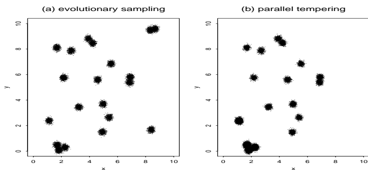
FIGURE 11.2. Scatterplots of the first 100,000 iterations of (a) the EMC algorithm and (b) parallel tempering.
