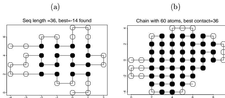
FIGURE 4.1. Configurations of two black-white bead chains with length 36 and 60, respectively. Configuration (a) has the minimum energy (verified by Unger and Moutl), whereas (b) has a total favorable contacts of 36, the optimal one we have obtained. Its true minimum energy is unknown.
