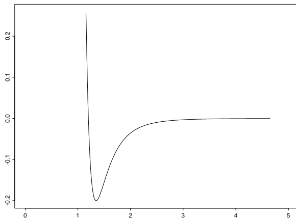
FIGURE 1.2. A plot of the Lennard-Jones function.
