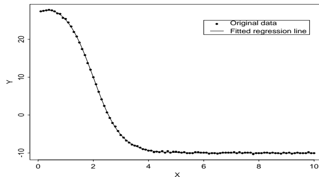
FIGURE 11.4. The original data overlaid by the MAP estimate (found by the EMC algorithm) of the unknown function.
