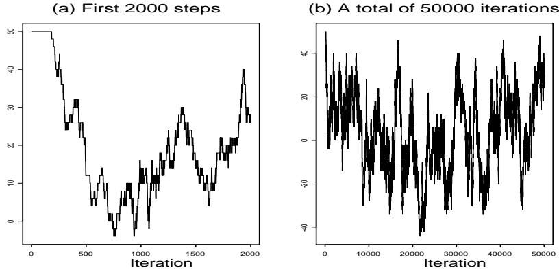
FIGURE 5.2. Simulation of the 1-D Ising model. The trace plots of (a) the first 2000 steps and (b) the total of 50,000 steps.
