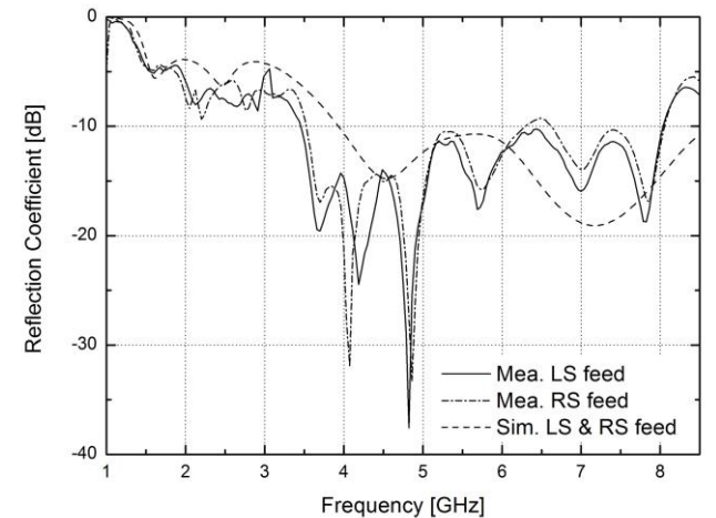
Fig. 7. Simulated and measured reflection coefficients of slotline feed.
