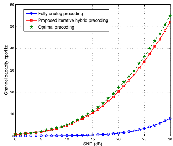
Fig. 4. Capacity comparison for an NM \times K = 128 \times 32 ( M = 4 ) mmWave massive MIMO system.
