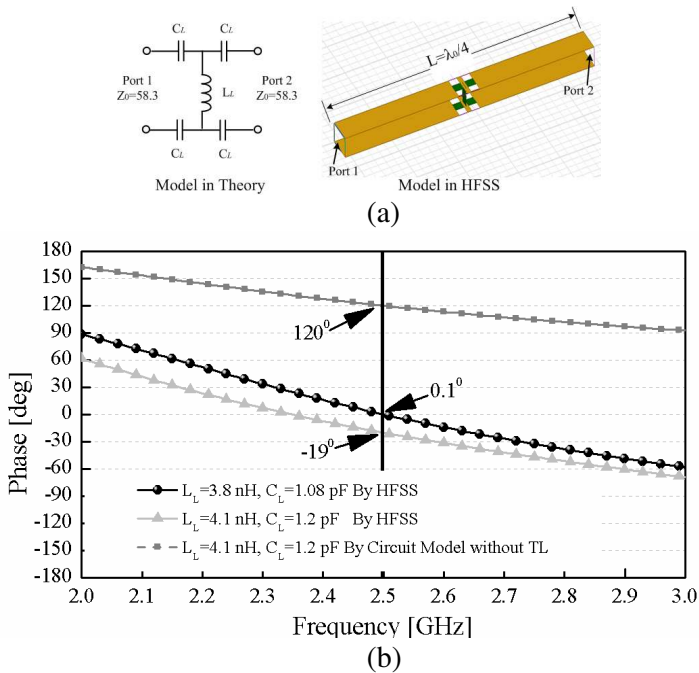
Figure 3. (a) Circuit model without TL and simulated model in HFSS. (b) Phase shift varied with frequency.
